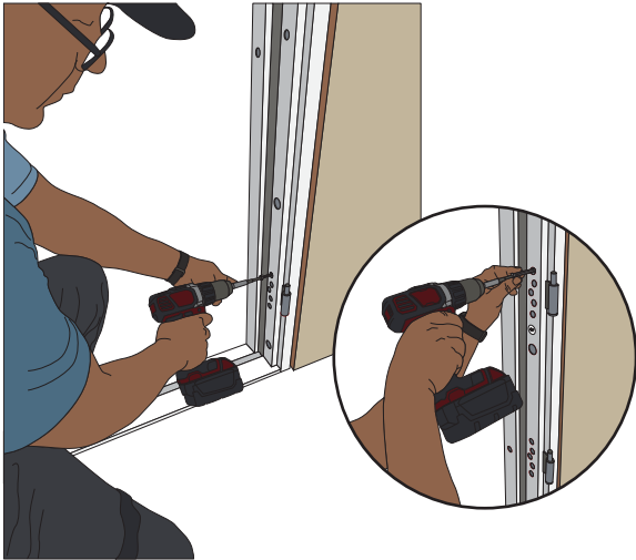
STEP 7. Fix the door frame (hinge side) to the wall using bolts.
