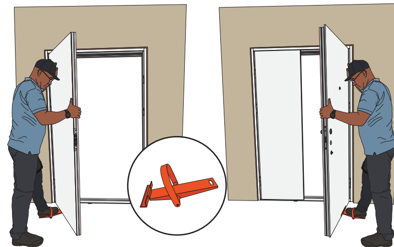
STEP 9. Both door leafs is hanged on the hinges using lever. Then align the door frame so that both door leafs and the frame are in the same plane.
